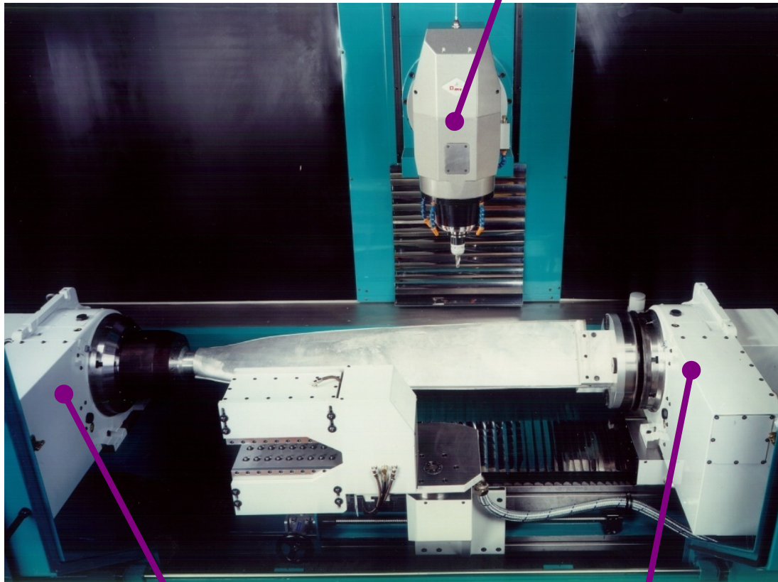
Testa Verticale con Motorspindle Vertical Milling Head with Motorspindle
